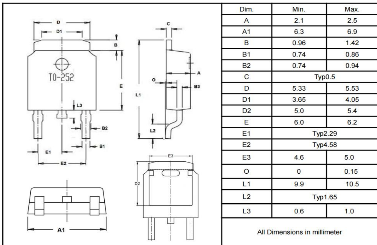
T0-252
